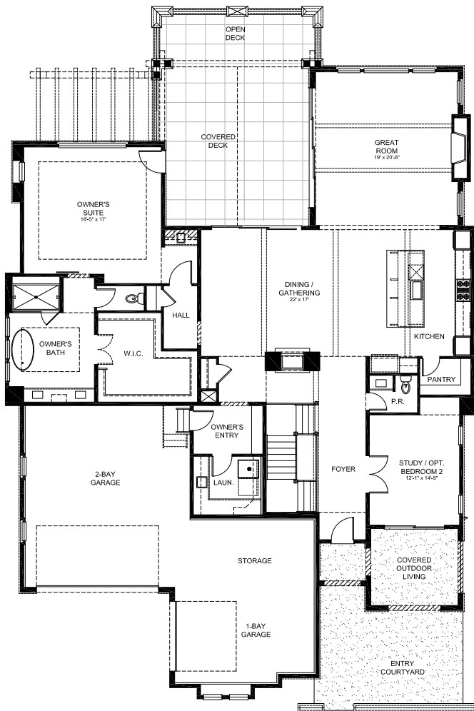
Main Level Floor Plan 2761 Sq. Ft.
