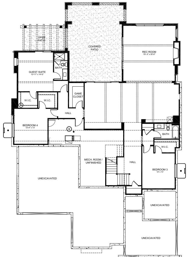
Lower Level Floor Plan 2662 Total Sq. Ft.
